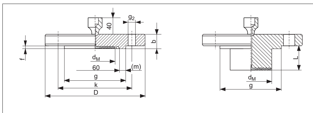
Process connection PMP75, EN/DIN flange with flush-mounted process isolating diaphragm, material AISI 316L
