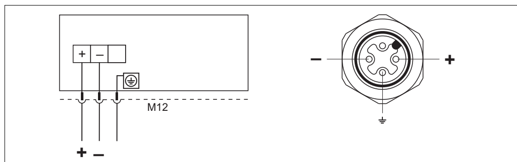
Left: electrical connection for devices with M12 plug
