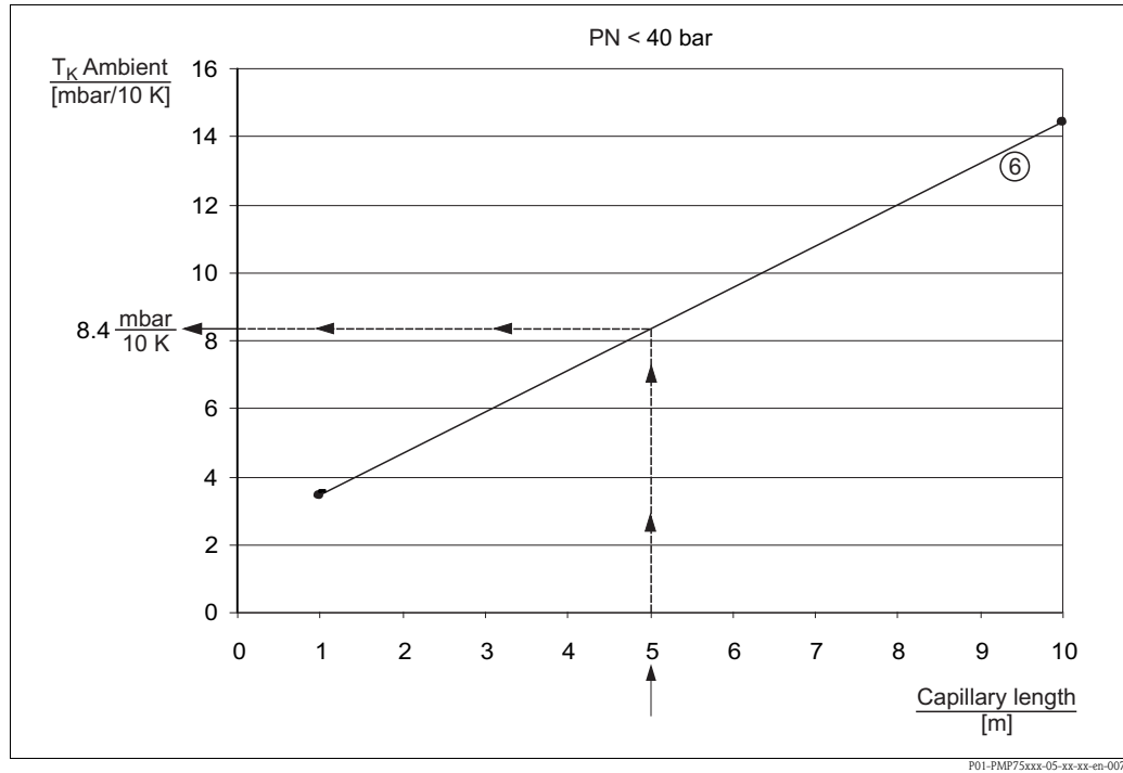
Diagram T_K \text{ Ambient} dependent on the capillary length for PMP75, PN < 40 bar
