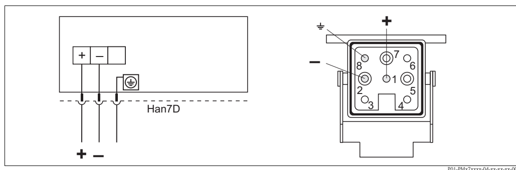
Left: electrical connection for devices with Harting plug Han7D
