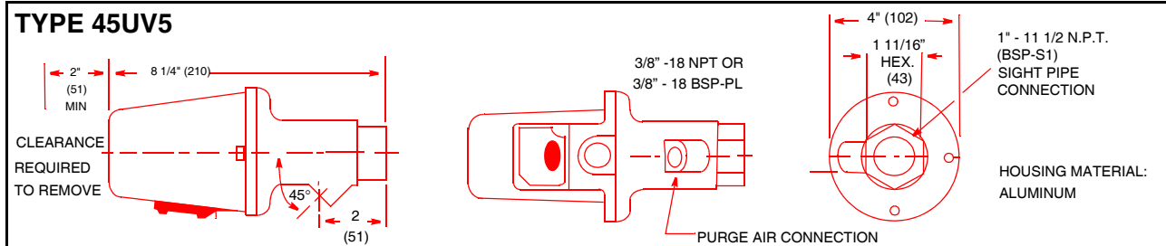
FIGURE 2. 45UV5 SCANNER IN CENELEC HAZARDOUS AREA HOUSING
