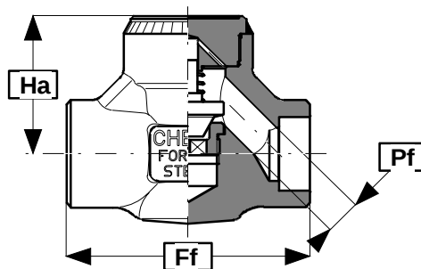
Piston (.P4..I)
