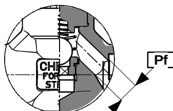
Ball (.B4..I)
