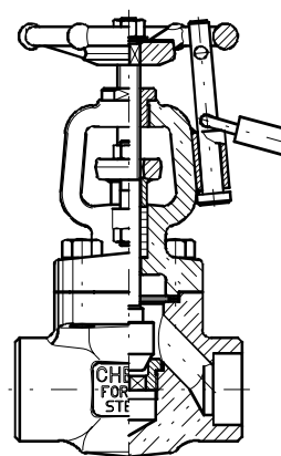
Locking device
