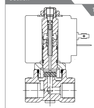
Coil 8W
