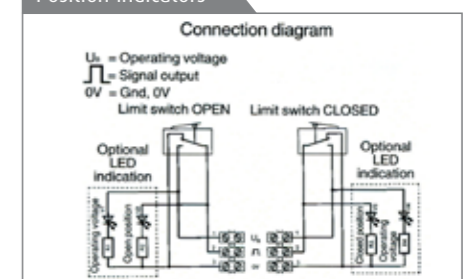
Position indicators
