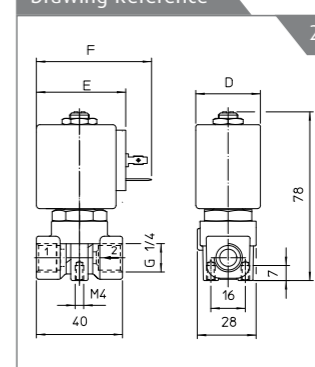
Coil 8W
