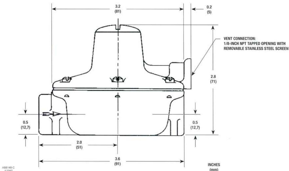
Figure 3. Dimensions
