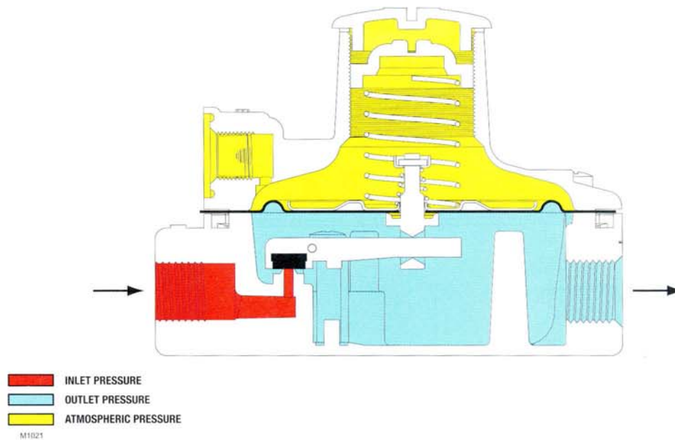
Figure 2. Operational Schematics
