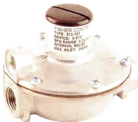
Figure 1. Type 912-101 Regulator
