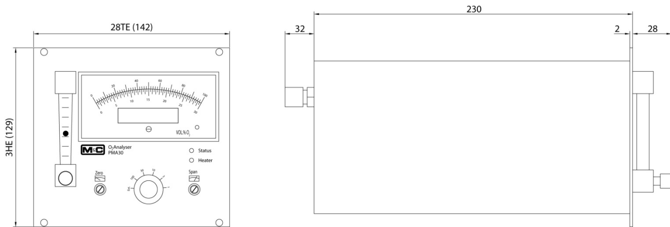
Figure 1 Dimensions PMA30
