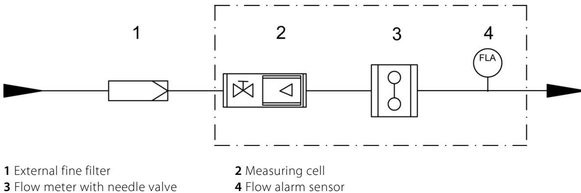
Figure 5 Gas flow diagram PMA30
