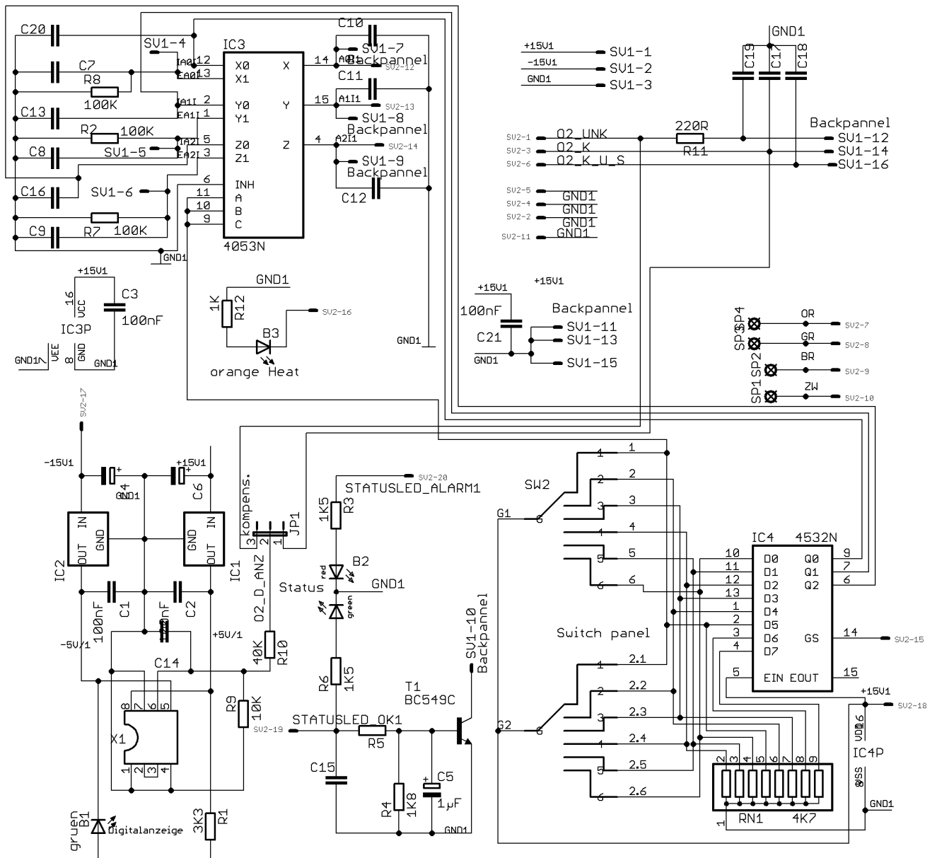
Figure 15 Circuit diagram PMA30 front board
