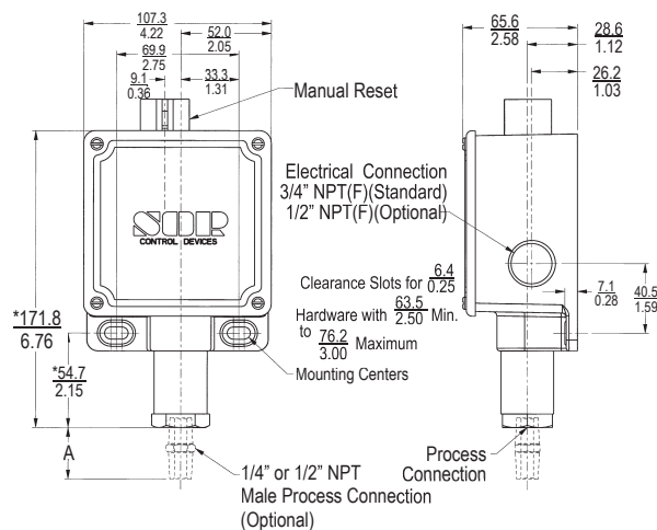
Designators: RB Manual Reset Piston Numbers 5, 6, 1, 9, 56
